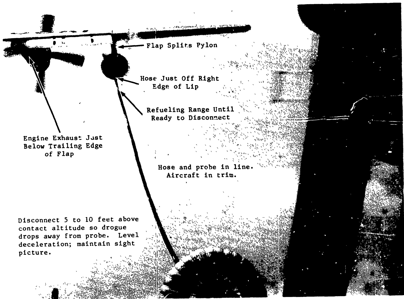
Photo 5. Right Disconnect Position
