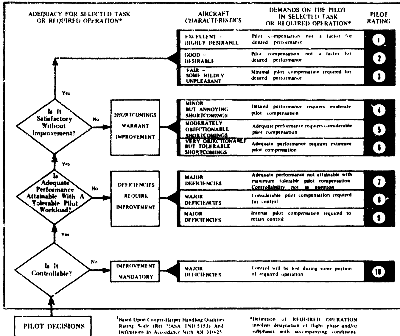
Figure 1. Handling Qualities Rating Scale
