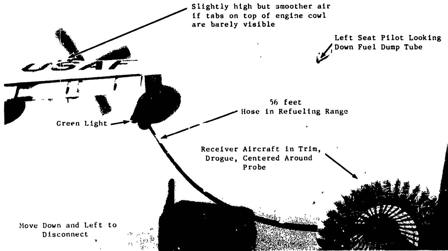
Photo 4. Right Refueling Position
