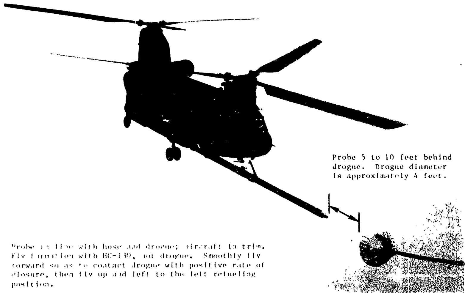
Photo 3. Left Precontact Position as Viewed from HC-130
